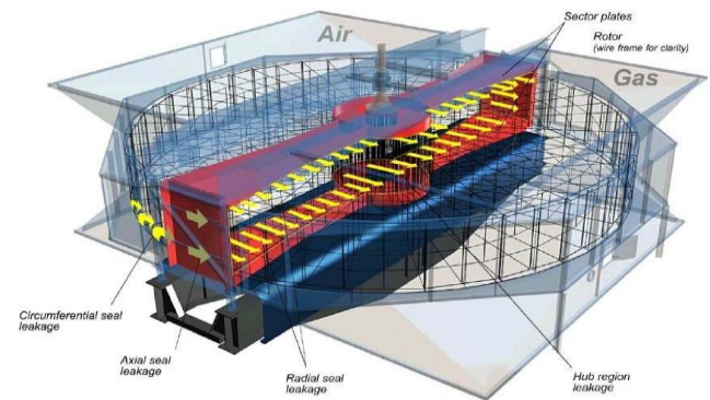
Fig 2: Ljungstrom Air Preheater (3D view)
